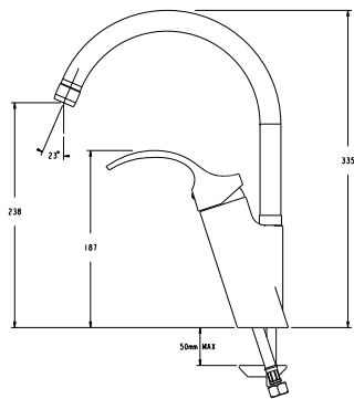
AU: 102770 NZ: 564582 Wave™ kitchen mixer: pg. 73
