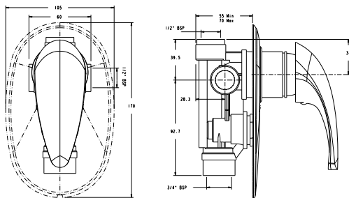
AU: 102771 NZ: 584584 Elosis concealed shower or bath mixer: pg. 60
