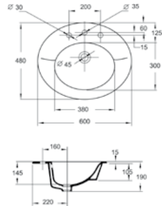
AU: 073367 NZ: 526998 single-hole AU: 073368 NZ: 585974 three-hole Presqu'île™ 600mm self-rimming basin: pg. 45
