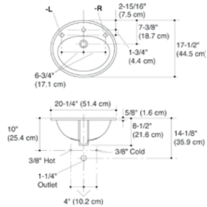
AU: 115274 NZ: 586007 single-hole AU: 115275 NZ: 586008 three-hole Pennington 514mm self-rimming basin: pg. 45
