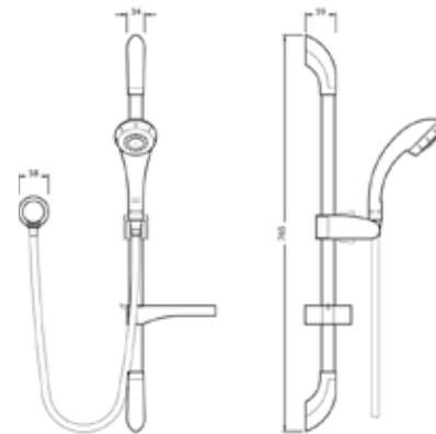
AU: 115117 NZ: 586155 Multifunction slide bar shower kit: pg. 71
