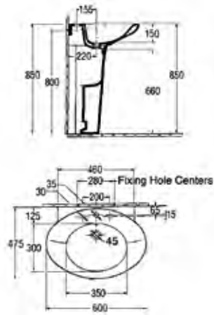
AU: 073326 / 115319 NZ: 507692 / 507128 single-hole AU: 073327 / 115319 NZ: 586123 / 507128 three-hole Presqu'île™ 600mm basin with pedestal: pg. 47
