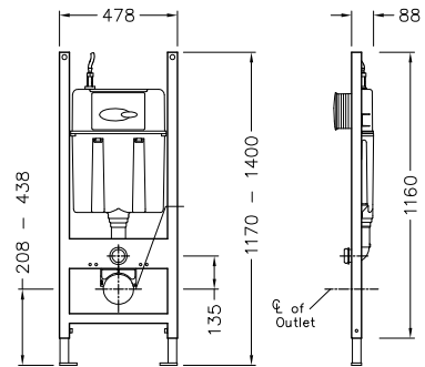
AU: 115288 NZ: 586121 (4.5/3 Litre) AU: 115287 NZ: 586122 (6/3 Litre) In wall tank and face plate, 88mm: pg. 31
