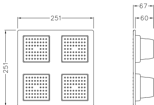
AU: 115312 NZ: 586013 WaterTile ® Rain shower panel: pg. 88
