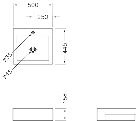
AU: 115082 NZ: 589009 single-hole AU: 115083 NZ: 589010 three-hole Parliament 500mm semi recessed basin: pg. 45
