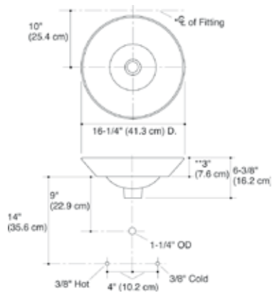
AU: 072722 NZ: 551893 Conical Bell™ Vessels 410mm basin: pg. 43
