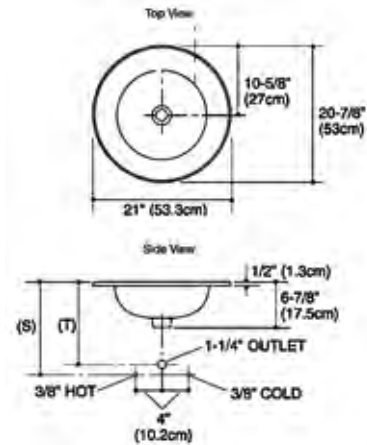
AU: 115078 NZ: 585971 Mythical Beasts ™ design on Camber ™ self-rimming 530mm basin: pg. 43
