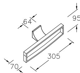
AU: 115066 NZ: 586102 Loure towel ring: pg. 96
