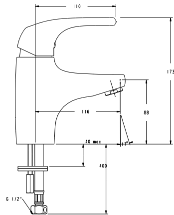
AU: 102777 NZ: 584506 Nateo single lever basin mixer: pg. 61
