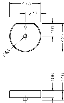
AU: 111123 NZ: 530557 single-hole AU: 115280 three-hole Chord™ Vessels 473mm basin: pg. 43
