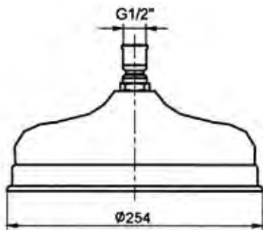
AU: 102795 NZ: 586151 Rainforest™ 254mm showerhead: pg. 71
