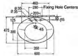
AU: 073326 / 073328 NZ: 507692 / 527006 single-hole AU: 073327 / 073328 NZ: 586123 / 527006 three-hole Presqu'île™ 600mm wall-mount basin with shroud: pg. 41
