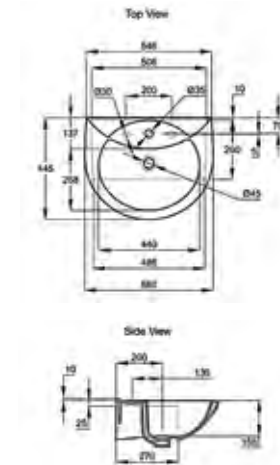
AU: 059125 NZ: 584502 single-hole AU: 059135 NZ: 586126 three-hole Odeon™ 560mm semi-recessed basin: pg. 45
