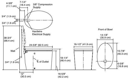
586120 Purist™ Hatbox toilet: pg. 27
