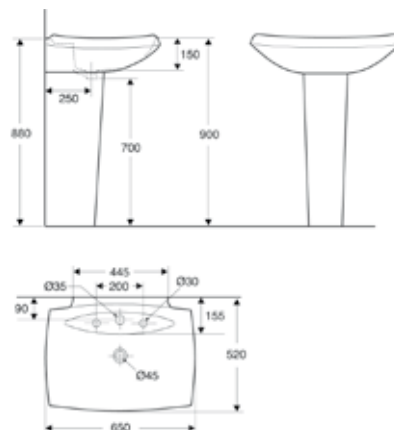
AU: 055579 / 064125 NZ: 530561 / 564215 Escale 650mm basin with pedestal: pg. 47
