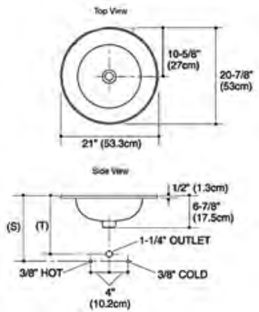
AU: 115277 NZ: 585959 Camber™ 533mm self-rimming basin: pg. 45
