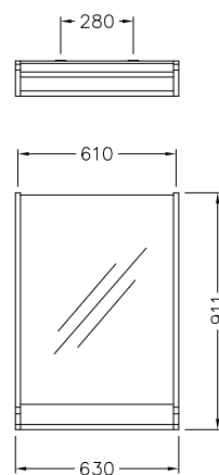
AU: 115068 NZ: 586161 Loure™ 610mm mirror and double towel bar: pg. 96
