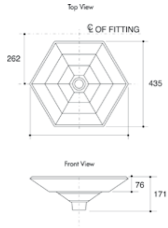
AU: 072802 NZ: 512493 Hex Strata™ Vessels 435mm basin: pg. 43
