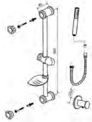
AU: 115116 NZ: 564577 Wave hand shower with slide bar kit: pg. 59
