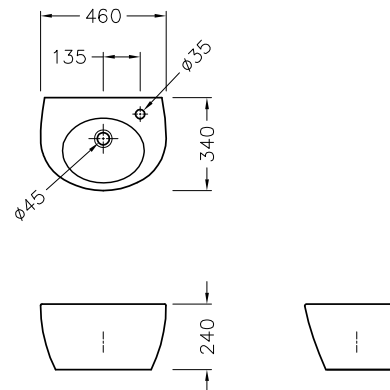
AU: 115264 NZ: 585996 Ove 340mm hand wash basin: pg. 41
