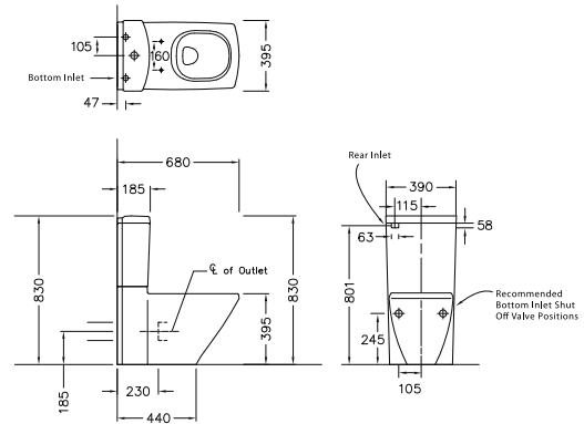
AU: 064127 NZ: 530571 Escale™ back-to-wall toilet with Quiet-Close™ seat: pg. 28
