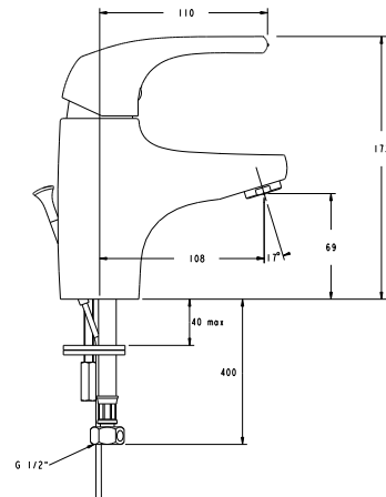
AU: 102778 NZ: 586061 Nateo™ single lever basin mixer with pop-up waste: pg. 61
