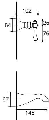
AU: 033214 NZ: 586141 Revival wall-mount bath set with traditional lever handles: pg. 67
