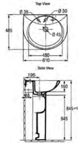
AU: 115269 / 115271 NZ: 518059 / 518071 single-hole AU: 115270 / 115271 NZ: 518070 / 518071 three-hole Odeon™ 610mm basin with pedestal: pg. 47
