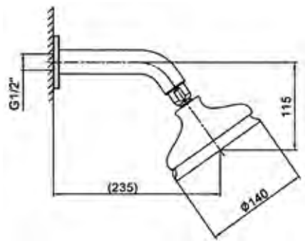
AU: 102796 NZ: 586390 Fairfax™ multifunction showerhead: pg. 70
