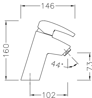
AU: 102782 NZ: 584507 Panache single lever basin mixer: pg. 62
