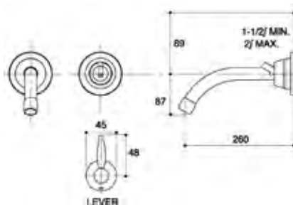
AU: 033204 NZ: 553154 Falling Water 260mm wall-mount basin mixer with 60° curved spout: pg. 57
