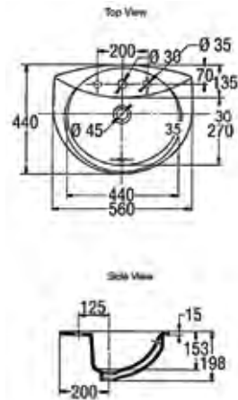
AU: 072450 NZ: 527000 single-hole AU: 072655 NZ: 586125 three-hole Odeon 560mm self-rimming basin: pg. 45
