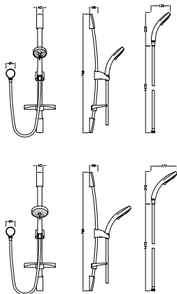
AU: 115027 NZ: 586077 / AU: 115028 NZ: 586392 Omega 90mm hand shower with slide bar kit 110mm hand shower with slide bar kit: pg. 71
