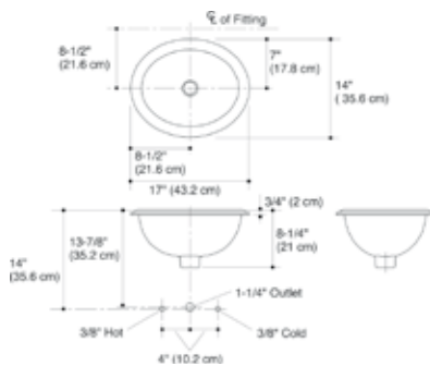
AU: 115077 NZ: 523988 Serpentine Bronze ™ design on Intaglio ™ self-rimming 432mm basin: pg. 43
