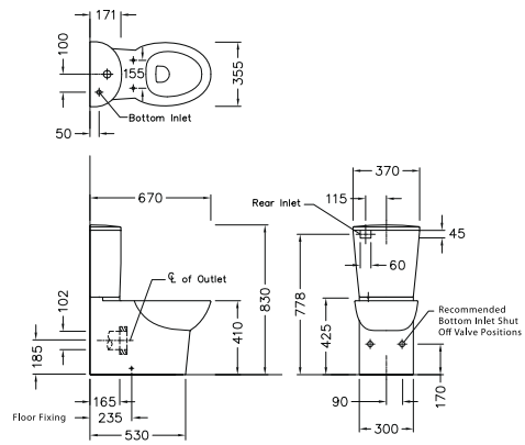
AU: 052254 NZ: 578633 Opiaz™ back-to-wall toilet with Quiet-Close Quick Release seat: pg. 29
