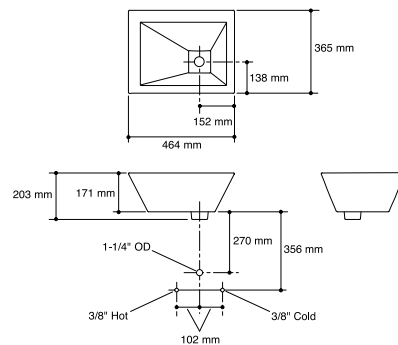
AU: 073116 NZ: 551892 Bateau ™ Vessels ™ 464mm basin: pg. 43
