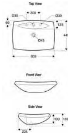
AU: 021063 NZ: 564218 Escale™ 600mm self-rimming basin: pg. 44
