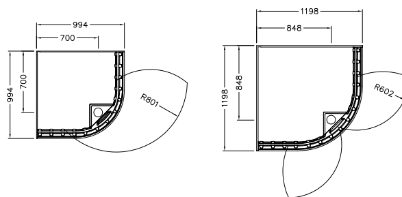
AU: 115010 / 115011 NZ: 527071 / 566230 1000 x 1000mm AU: 115012 NZ: 527072 1200 x 1200mm Trilogy ™ Round Corner shower : pg. 89
