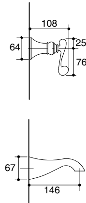
AU: 033211 NZ: 586140 Revival ® wall-mount bath set with scroll handles: pg. 67
