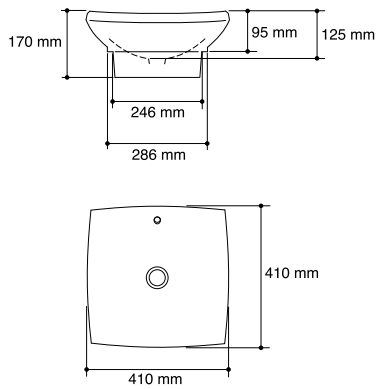
AU: 064129 NZ: 564212 Escale™ Vessels™ 410mm basin: pg. 43
