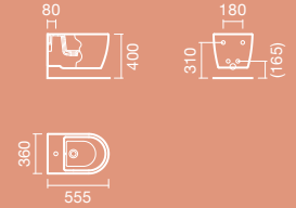
BIDET wall-mounted
