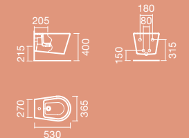
BIDET wall-mounted
