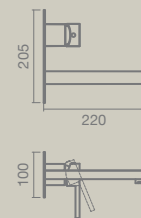
WASHBASIN wall-mounted
