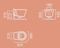
TOILET wall-mounted
