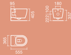
TOILET wall-mounted
