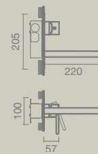
WASHBASIN wall-mounted
