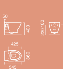
TOILET wall-mounted
