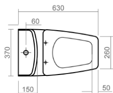
Close coupled pan and cistern
