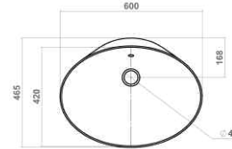
600mm countertop basin
