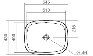
550mm inset vanity basin
