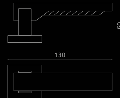
ARKADHT05F4OP9 Maniglia in cristallo ambra 24% Pb, molato a mano con mole a pietra. Montatura in ottone cromato. Hand bevelled in stone, 24%Pb amber crystal door handle. Chrome plated brass base.
