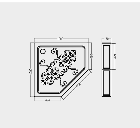
ARABESQUE PENTA (100X100)
