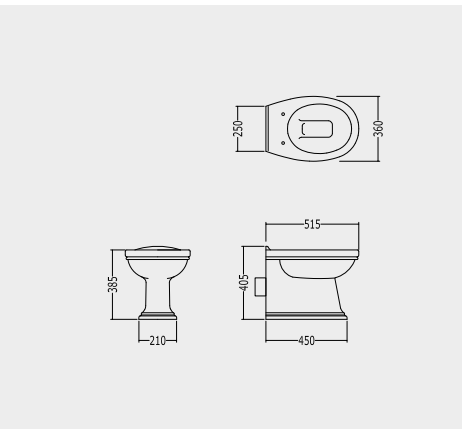
ROSE BACK TO WALL W.C. PAN
